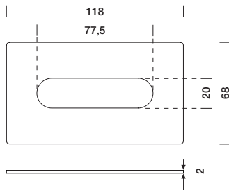
89 51 241 Support plate ETEREA large
