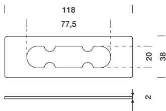
89 51 240 Support plate ETEREA medium
