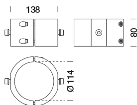
8951050 Connection to the pole 114 mm Ø
