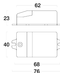
8956116 Dimmable driver for maximum 3 luminaires (250mA) (250/700mA - 30/40W) IP20 1- 10V+Push+DALI
