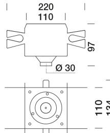
8945110 Recessed box E2 - reinforced concrete
