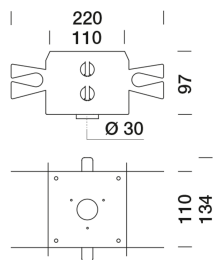
8945105 Recessed box E2 - plaster
