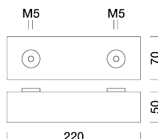
8952022 Junctuion box for two floodlights (Connector 8917004 included)
