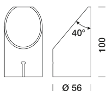
8935220 Visor
